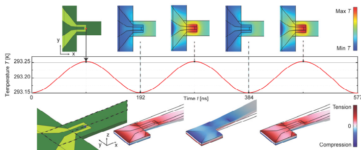
Figure 1. Nanoactuator temperature change in time due to an input current of 1 mA at 5.2 MHz. The temperature field and stress/strain field at indicated time points are shown on the top and bottom of the figure, respectively.
